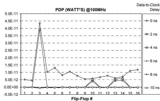
(b) Using Clk2Q delay.
