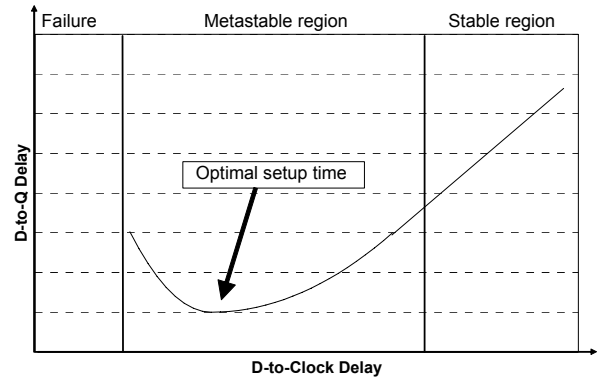
Figure 1 Flip-Flop regions of operation.
