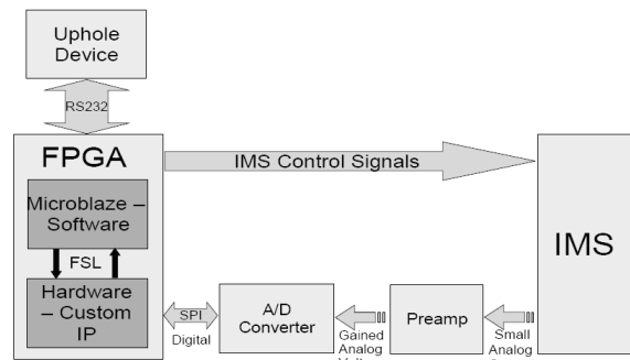
Figure 3. IMS electrical sub-system
