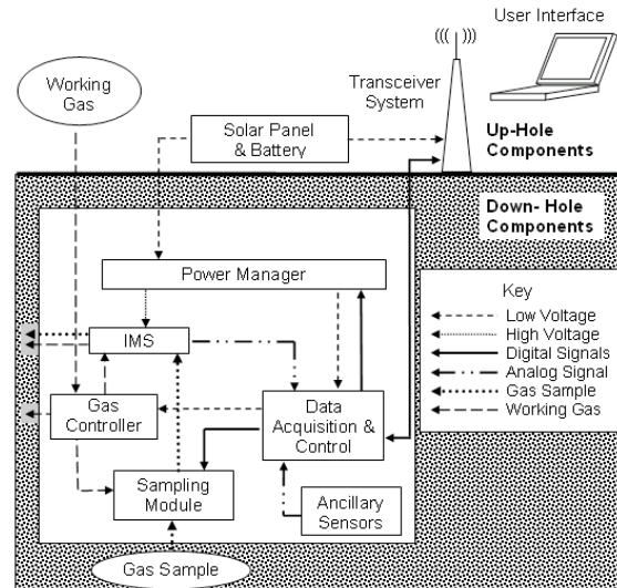
Figure 1. IMS sensor system block diagram.
