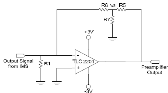
Figure 4. Preamp Circuit Diagram [5]
