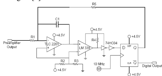
Figure 5. Delta Sigma Modulator [5]
