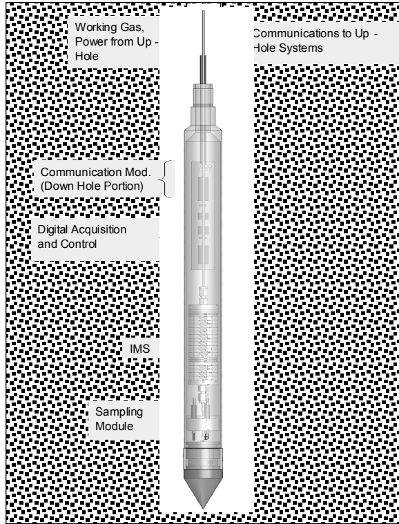
Figure 2. Layout of the IMS sensor system in probe housing.
