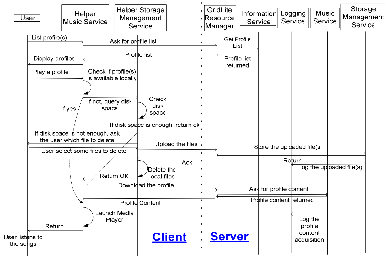
Figure 5. Sequence Diagram of Music Service
