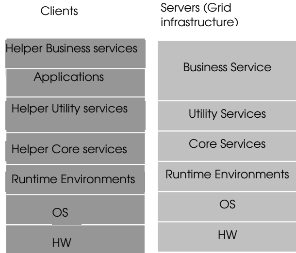
Figure 2. GridLite Software Stack
