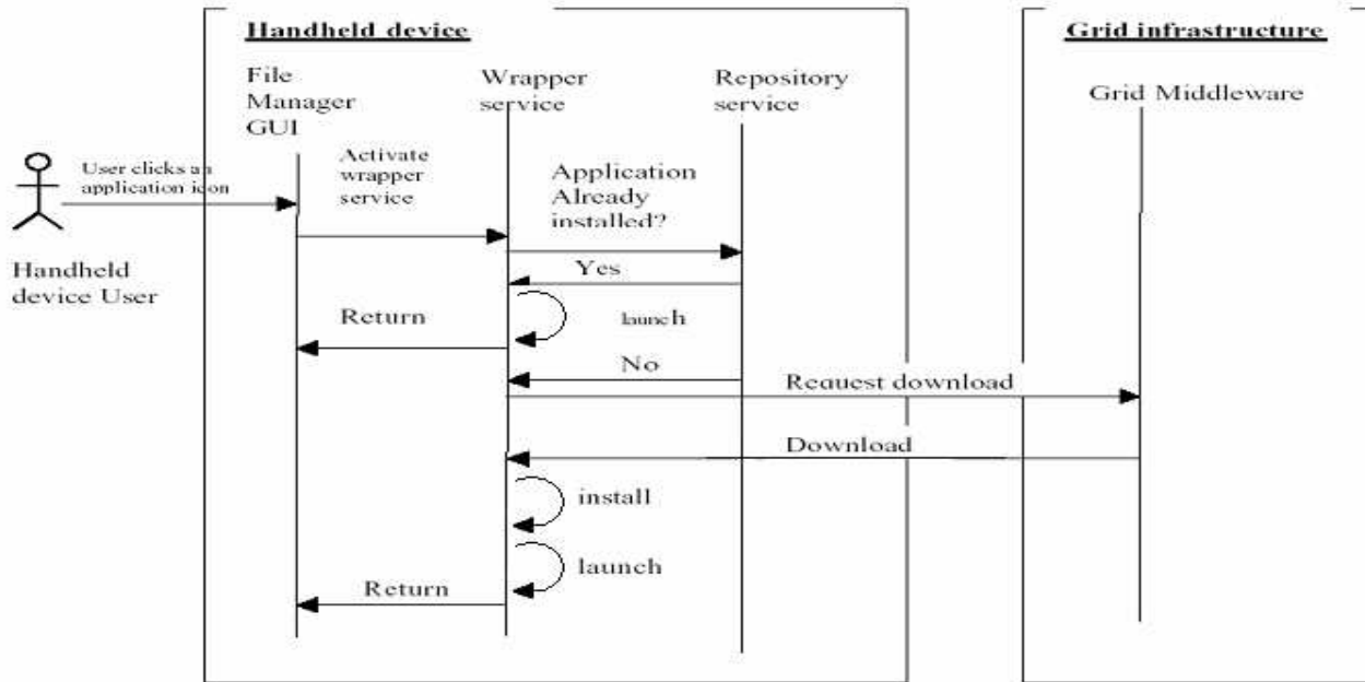
Figure 4. Sequence Diagram of Application Management Service
