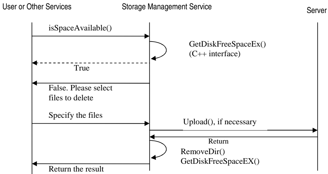
Figure 3. Sequence Diagram of Storage Management Service
