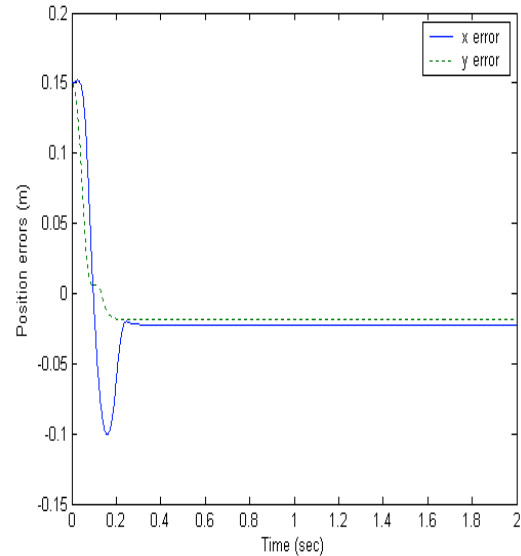
Fig. 5. Positions error with respect to the reference values. Solid: error in x, dotted: error in y.
