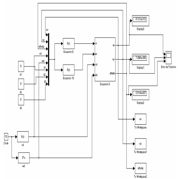
Fig. 9 Simulink block diagram of the controller.
