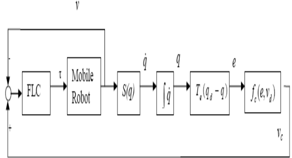
Fig. 2. Tracking control structure
