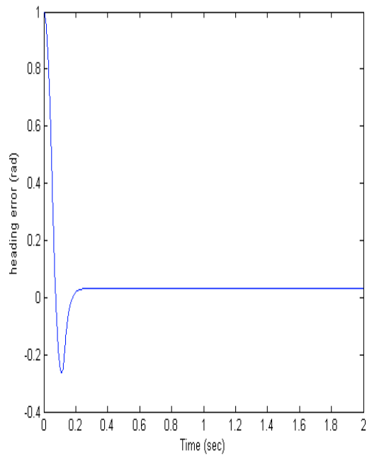
Fig. 6. Orientation error with respect to the reference values.
