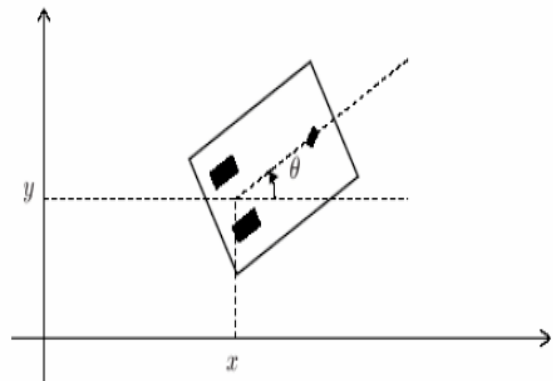
Fig. 1. Wheeled mobile robot.
