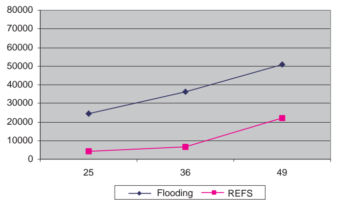
Fig. 2. The number of transmitted packets in function of the number of nodes for plain flooding and the REFS algorithm
