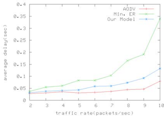
Figure 6. End-to-end delay for traffic rate
