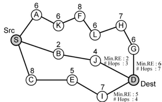
Figure 4. A sample network for establishment of routing paths
